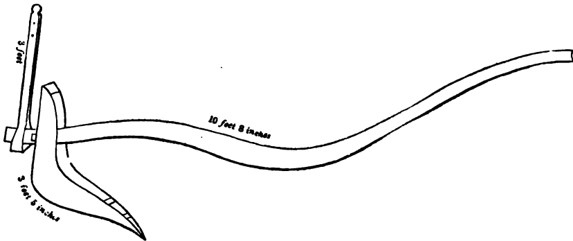
CHATAKRAL PLOUGH.
